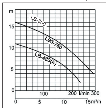
Pumpekurve
